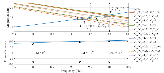
Fig. 11. Screening results for series resonance of different parallel PIC cases.
