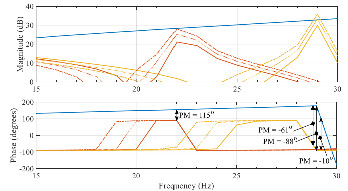
Fig. 12. Screening results for parallel resonance of parallel PIC cases.
