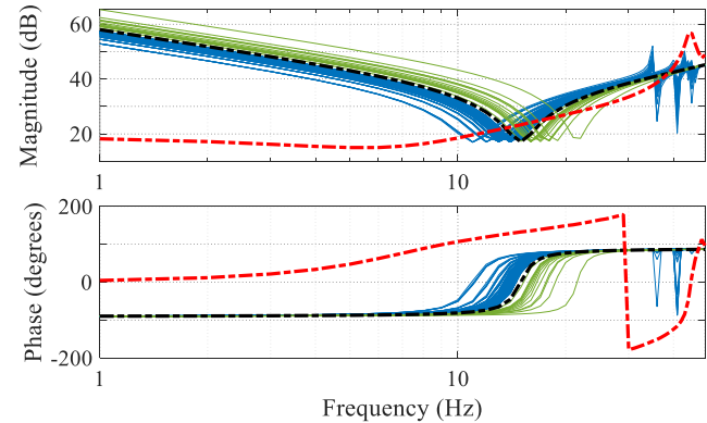
Fig. 17. Positive sequence impedance responses of DFIG (red) and the modified IEEE 39 bus system. Black curves represent the response of the N-5 grid using classical compensation. Green and blue curves represent respectively series and parallel PIC.
