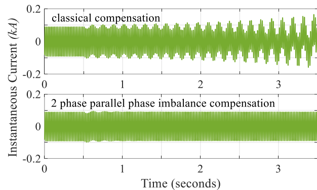
Fig. 15. Phase C instantaneous currents for 19% compensation.
