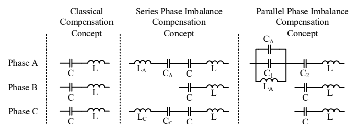
Fig. 1. Overview of the classical and series and parallel phase imbalance compensation schemes.
