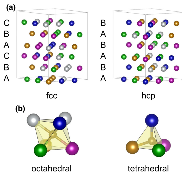
Fig. 1 (a) Simulation cells with 54 atoms for the fcc and the hcp phases. (b) Interstitial sites considered for N. Spheres in different colors represent different elements. Visualization is performed using the VESTA code [90]
