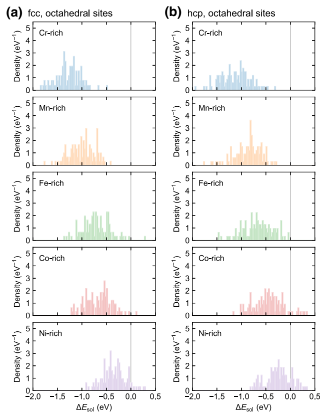
Fig. 4 Distributions of the computed solution energies \Delta E_{\text{sol}} of N atoms at octahedral sites in M -rich INN local chemical environments ( M = \text{Cr, Mn, Fe, Co, Ni} ) for the a fcc and the b hcp phases of CrMnFeCoNi
