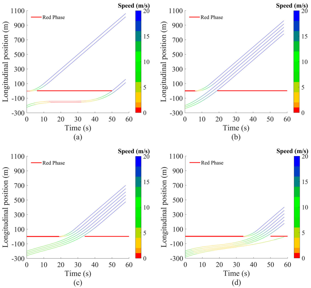
Figure 6. Longitudinal Position under Scenario 3. (a) first movement (b) second movement (c) third movement (d) fourth movement.
