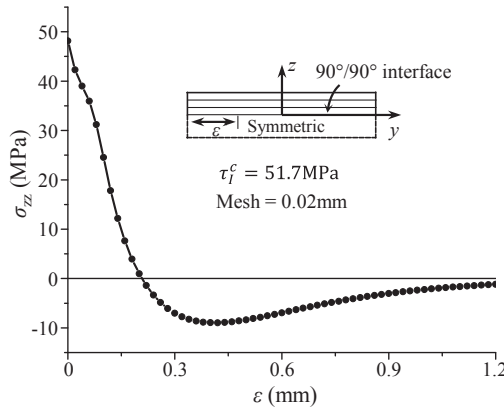
Fig. 9. Numerical results of free-edge delamination analyses.
