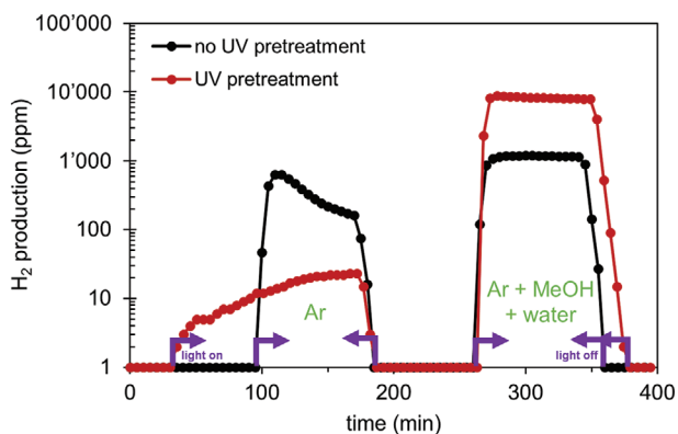
Figure 3. Amount of absolute hydrogen production in ppm produced over time by an as-synthesized (black) and a UV pretreated (red) TiO 2 -Pd aerogel. Hydrogen production is depicted in a logarithmic scale. The illumination time is indicated with violet arrows. During the first illumination phase, only Ar gas flows through the aerogel. During the second illumination phase, the Ar gas is humidified with MeOH and water.
