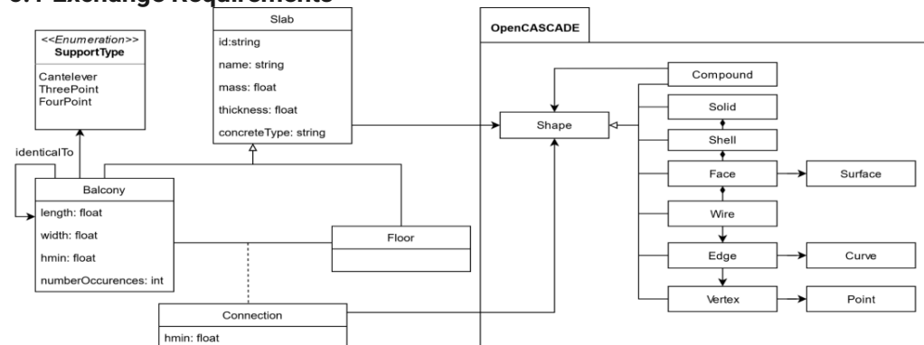
Figure 7. Conceptual data model of the extraction. Balcony and Floor are both subtypes of a type Slab that roughly corresponds to IfcSlab (but can be other types of IFC elements). Connection describes the geometric overlap between Balcony and Floor. In the vertical sense this is summarized as hmin.
