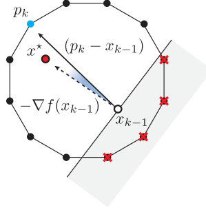
Fig. 1. Schematic illustration of the steepest descent permutation discussed in Observation 2. The black dots with a red cross are the extreme points that are non-descent directions. Frank-Wolfe with f(x) = (1/2)\|x^* - x\|_2^2 chooses the extreme point p_k (i.e., the permutation) that minimizes the angle between (p_k - x_{k-1}) and -\nabla f(x_{k-1}) = (x^* - x_{k-1}) .
