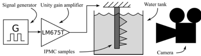
Fig. 6. Experimental set-up for measuring the quasi-static deflections of IPMC samples with different geometries.
