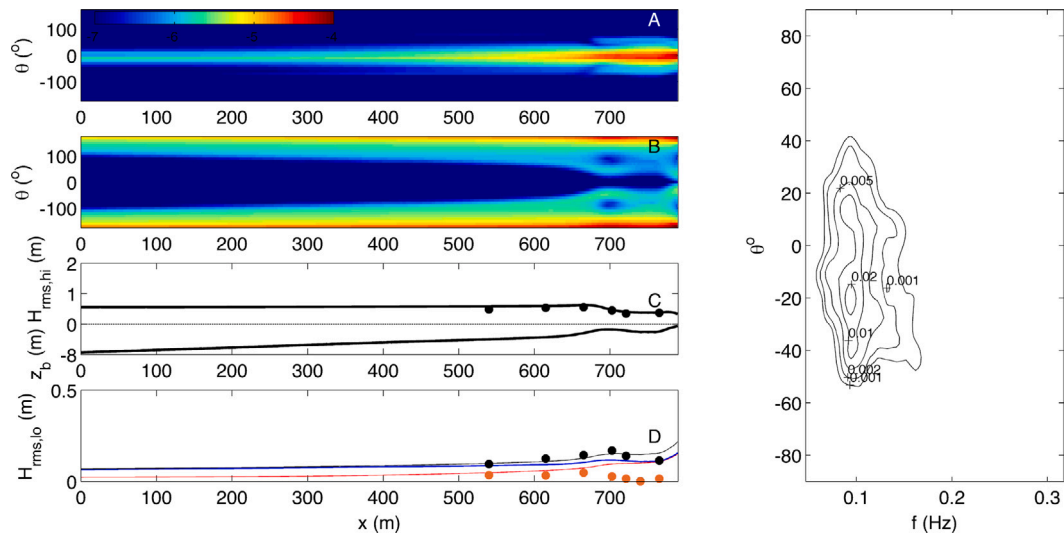
Fig. 6. Left panels: Wave transformation on October 15 at 10 pm. Panel A: Frequency-integrated WGF infragravity variance (logarithmic color scale in m^2/\theta ). Panel B: Reflected infragravity variance. Panel C: H_{rms,hi,c} (black line) compared with observations H_{rms,hi,m} (black dots). Panel D: WGF H_{rms,lo,f} (red line) compared with bound infragravity wave height (orange dots). Total predicted infragravity height H_{rms,lo,c} (black line) compared with observations of H_{rms,lo,c} (black dots). Reflected H_{rms,lo,r} given as a reference (blue line). Right panel: Sea-swell frequency-directional spectrum at FRF 8-m array for October 15 at 10 pm. Direction \theta is with respect to the shore normal. (For interpretation of the references to color in this figure legend, the reader is referred to the web version of this article.)
