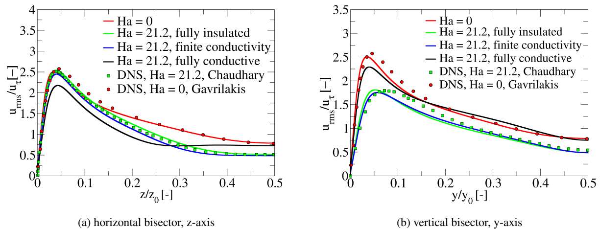
Figure 5: RMS profiles
