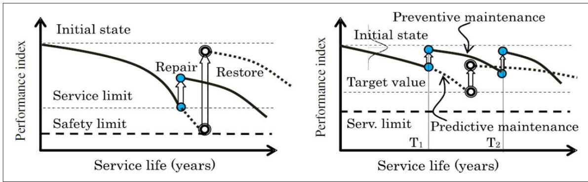
Figure 3 Two types of maintenance philosophies (a) corrective maintenance and (b) preventive and predictive maintenance [2]
