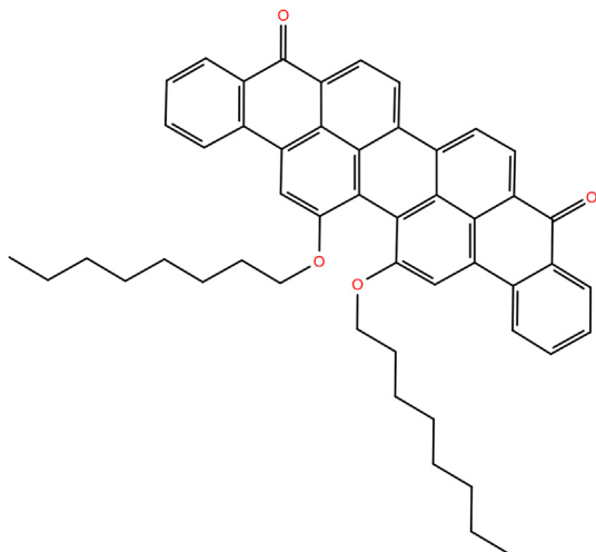
Fig. 1. 2-dimensional structure of the asphaltene model compound, i.e., Violanthrone-79 considered within this study. Aromatic core, polar-hetero-atoms, i.e., oxygen and two side chains are shown.
