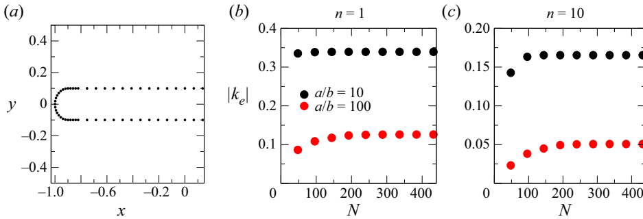
Figure 10. (a) Example of the discretisation of a n = 1 surface with N = 96 . (b,c) Effective aspect ratio |k_e| versus the number of discretisation points N for platelets with \lambda = 20 nm, a/b = 10 or a/b = 100 , and either n = 1 (b) or n = 10 (c).
