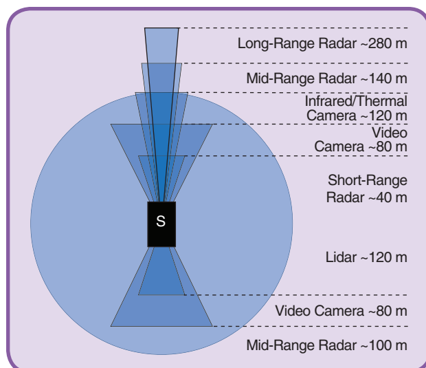
FIG 3 Illustration of a possible sensor configuration on a mobile sensing platform.
