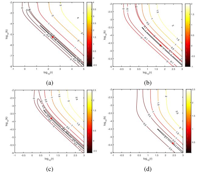
FIGURE 4. Dependence of the RMSE fitting errors on the values of r and k : (a) 385nm, (b) 405nm, (c) 415nm, (d) 450nm. Contours: \log_{10}(\text{RMSE}) ; Stars: the NLS estimates.
