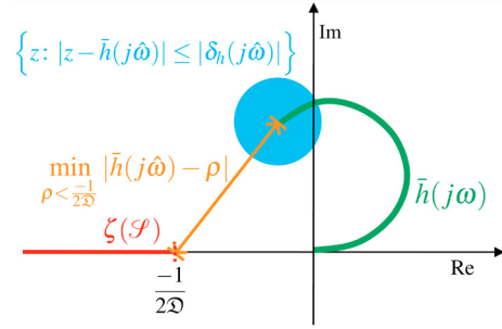
Figure 1. Visualisation of the robust stability condition in Lemma 1. Nyquist diagram of the nominal transfer function \bar{h}(j\omega) (green), uncertainty disk centred at \bar{h}(j\omega) representing \delta_h(j\omega) at the frequency \omega (cyan), set \zeta(\mathcal{S}) (red) and distance of \bar{h}(j\omega) from the set \zeta(\mathcal{S}) (orange). For all \omega \in \mathbb{R}^+ , the distance of \bar{h}(j\omega) from the set \zeta(\mathcal{S}) needs to be larger than the uncertainty radius \delta_h^{\text{max}}(j\omega) \geq |\delta_h(j\omega)| .
