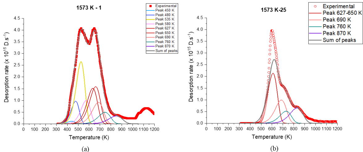
Figure 7. 4. Fitting of TDS spectra obtained for ODS 12 Cr steel samples (a) 1573 K-1, measured 1 day after \text{D}_2 exposure and (b) 1573 K-25, measured 25 days after exposure.
