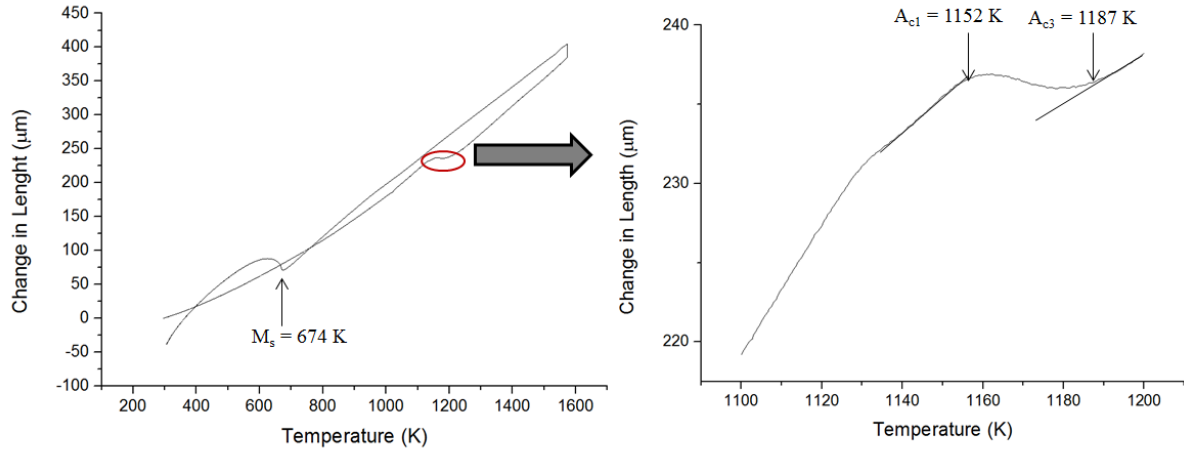
Figure 3. 5. Dilatometry curve obtained for the ODS Eurofer steel with a heating rate of 1 \text{ K.s}^{-1} , until 1573 \text{ K} . After holding for 5 \text{ min} at the maximum temperature, the sample was cooled, at an average rate of 0.8 \text{ K.s}^{-1} , by switching-off the HF power system of the dilatometer.
