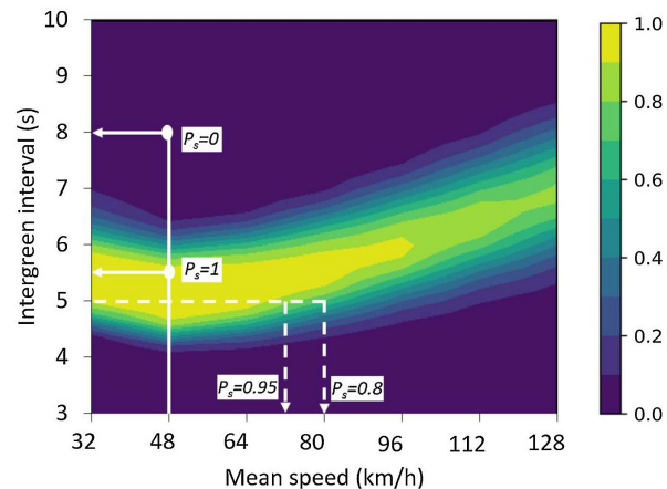
Fig. 8. Mapping the intergreen intervals for system survivability (COV = 10%).
