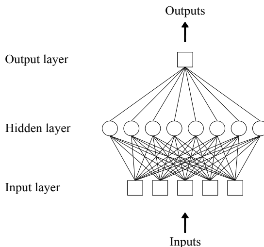
Figure 1. General schematic of a feed-forward artificial neural network
