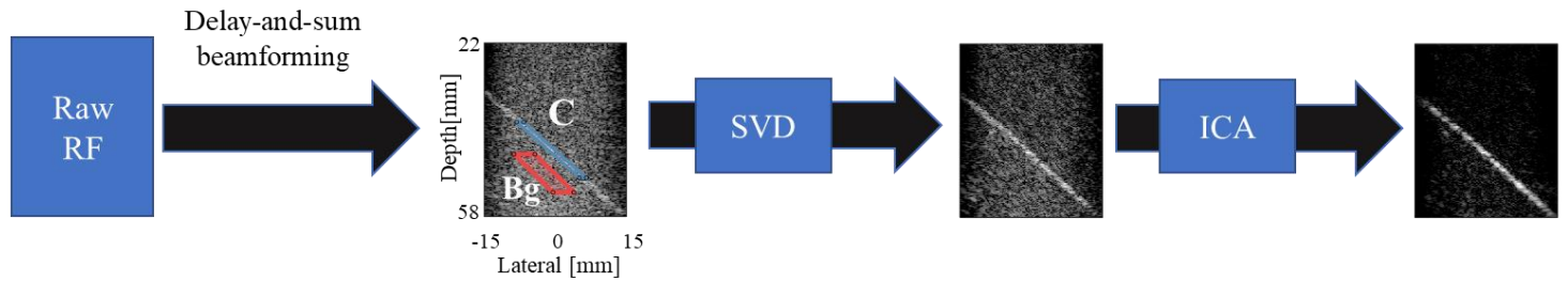
Fig. 2. Overview of the BSS filter framework. Example of regions of interest for calculating CBR. C (blue box) was used for contrast signal strength and Bg (red box) was used for background signal strength. Image is displayed with 40dB dynamic range.
