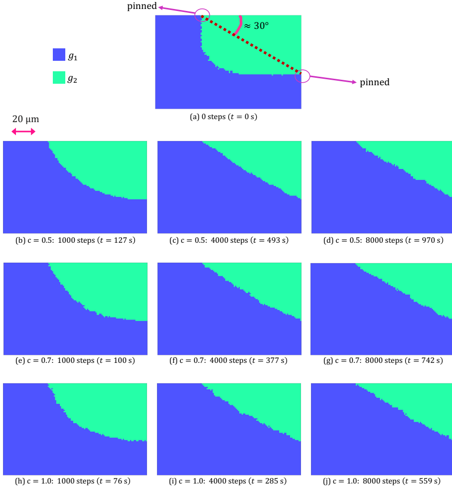
Figure 3.15: Bicrystal RVE at 1000 °C simulated in Sq(1,2) with confined boundary. The maps show the evolution at (a) 0 time steps - 0 s (b) 1000 time steps for c = 0.5 (c) 4000 time steps for c = 0.5 (d) 8000 time steps for c = 0.5 (e) 1000 time steps for c = 0.7 (f) 4000 time steps for c = 0.7 (g) 8000 time steps for c = 0.7 (h) 1000 time steps for c = 1.0 (i) 4000 time steps for c = 1.0 and (j) 8000 time steps for c = 1.0 .
