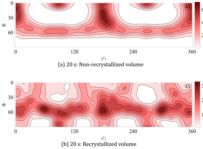
Figure 2.6: Samples 3 to 5: ODF quantified and plotted in section \varphi_2 = 45^\circ for the material after 20 s annealing of at 600^\circ\text{C} where (a) corresponds to the (still) deformed material and (b) to the recrystallized areas.
