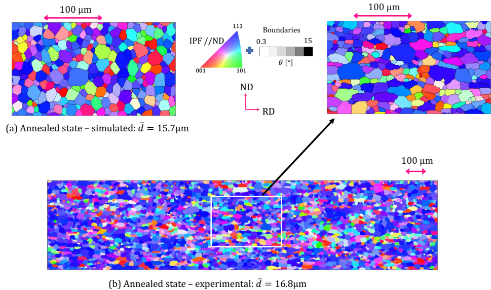
Figure 4.6: Recrystallized cold-rolled IF steel; (a) the simulated microstructure (b) the experimental measurement. The annealed state corresponds to the end of the heat treatment shown in Fig. 4.3.
