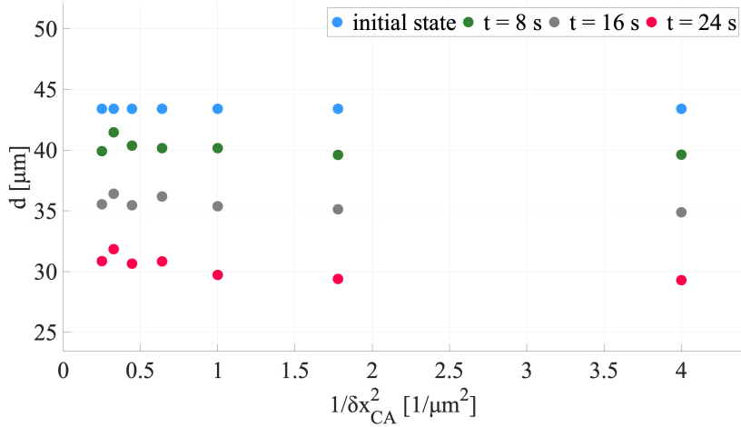
Figure 3.21: Dependency of grain growth kinetics on resolution and grid-spacing in Sq(1,2): the simulations are done using c = 0.7 at 1000\text{ }^\circ\text{C} . The grain diameter is shown for the embedded circular grain at different times as a function of the resolution/grid-spacing.
