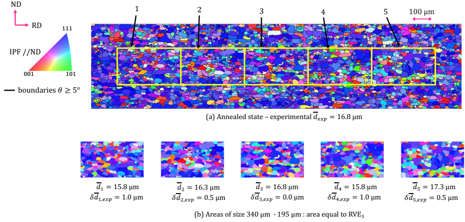
Figure 5.7: Method used to calculate \delta\bar{d}_{RVE_3} where (a) the experimentally measured microstructure (b) the subdivision in areas equal to the size of RVE_3 .
