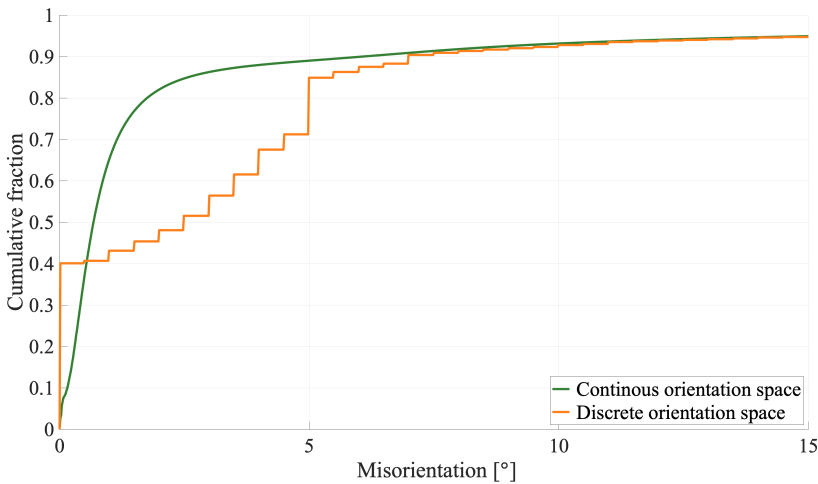
Figure A.2: Cumulative distribution of misorientation with \theta \leq 15^\circ for the cold-rolled IF steel microstructure.
