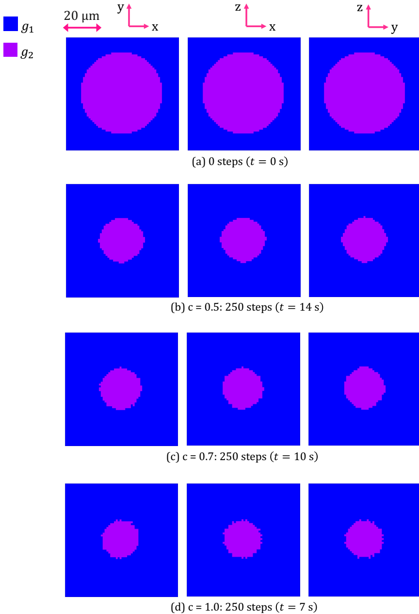
Figure 3.19: Bicrystal RVE at 1000 °C in Cub(2,2): The maps show the xy , xz and yz (middle) cross sections at (a) 0 time steps - 0 s (b) 250 time steps for c = 0.5 (c) 250 time steps for c = 0.7 (d) 250 time steps for c = 1.0 .
