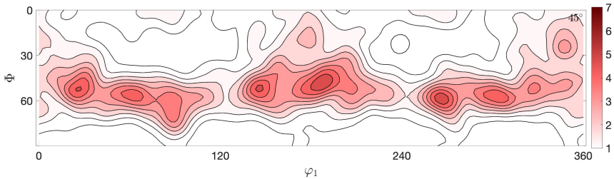
(b) RVE_2 : for V_{HAGB}^{rx} = 71\% of recrystallized volume
