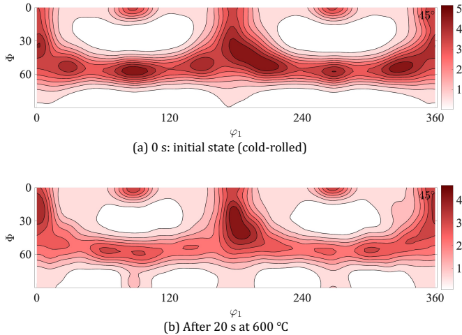
Figure 2.5: Samples 3 to 5: ODF quantified and plotted in section \phi_2 = 45^\circ for (a) the initial condition after cold rolling and (b) after 20 s of annealing at 600 °C.
