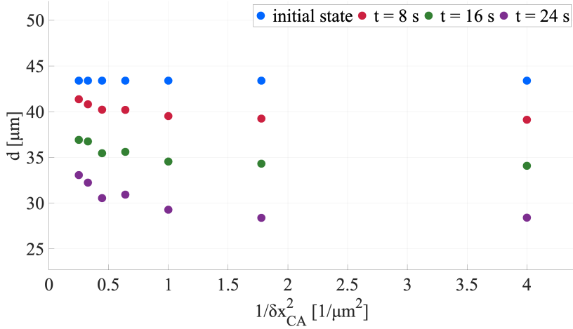
Figure 3.20: Dependency of grain growth kinetics on resolution and grid-spacing in Hex(1,1) the simulations are done using c = 0.7 at 1000\text{ }^\circ\text{C} . The grain diameter is shown for the embedded circular grain at different times as a function of the resolution/grid-spacing.
