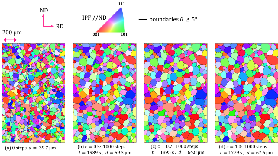
Figure 3.17: Polycrystal RVE at 800 °C simulated in grid Hex(1,1) shown at (a) 0 time steps (b) 1000 time steps - for c = 0.5 (c) 1000 time steps for c = 0.7 (d) 1000 time steps for c = 1.0 .
