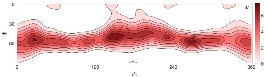
(c) Experimental annealed state - ODF \phi_2 = 45^\circ
