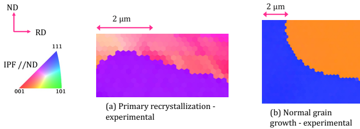
Figure 4.2: EBSD observations during the annealing of the IF-steel sheet. The phenomena depicted are (a) primary recrystallization - i. e. a recrystallized grain grows into a substructure (b) grain growth - i. e. two recrystallized grains have impinged.
