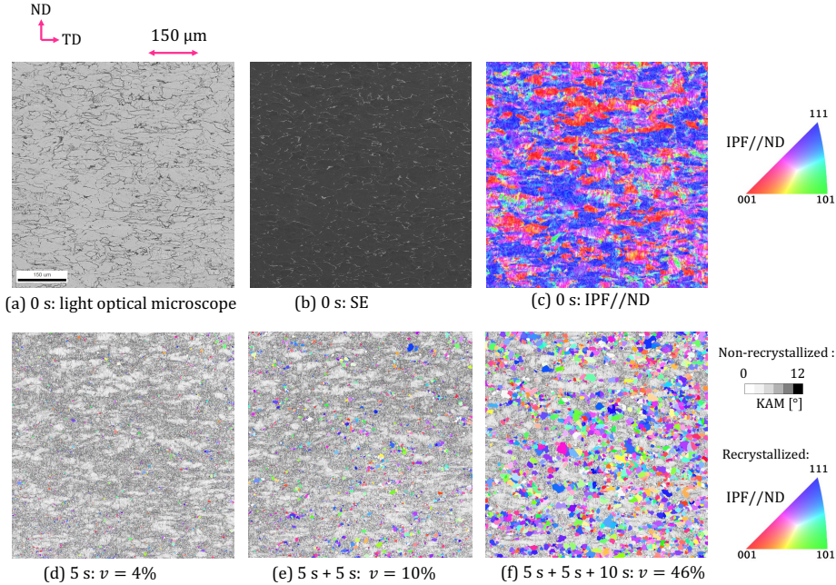
Figure 2.13: Sample 3: Initial microstructure and partially recrystallized states plotted with combined IPF and KAM maps. The scanned area is equal to 600\ \mu\text{m} \times 600\ \mu\text{m} and the recrystallized fraction is denoted by v .
