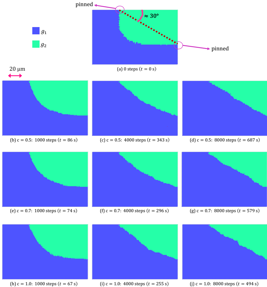
Figure 3.14: Bicrystal RVE at 1000 °C simulated in Hex(1,1) with confined boundary. The maps show the evolution at (a) 0 time steps - 0 s (b) 1000 time steps for c = 0.5 (c) 4000 time steps for c = 0.5 (d) 8000 time steps for c = 0.5 (e) 1000 time steps for c = 0.7 (f) 4000 time steps for c = 0.7 (g) 8000 time steps for c = 0.7 (h) 1000 time steps for c = 1.0 (i) 4000 time steps for c = 1.0 and (j) 8000 time steps for c = 1.0 .
