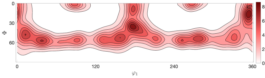
(a) Deformed state - ODF \phi_2 = 45^\circ
