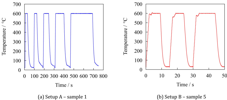
Figure 2.2: Temperature-time profile where (a) represents setup A, as measured for sample 1 (b) represents setup B, as measured for sample 5.
