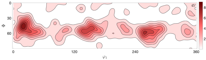
(b) Simulated annealed state - ODF \phi_2 = 45^\circ
