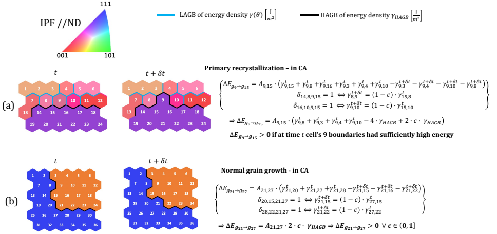
Figure 4.1: Cell switching scenarios in the CA. The two main cases that will occur when the algorithm is applied to a deformed microstructure discretized in a 2D hexagonal automaton grid are shown. The images depict the energy state before and after the re-orientation. In Figure (a) cell 15 (growing cell) belongs to a recrystallized volume (or large subgrain next to a HAGB) and might grow into cell 9 that belongs to a substructure. Although the migration increases the HAGB area, a positive driving force can still be found since the LAGB area decreases. Also, cell 15 has neighbours (i. e. cells 14 and 16) of the same orientation which can grow in the same direction (i. e. toward cells 8 and 10, respectively). In this case, only a part (i. e. 1 - c ) of the energy concerning the boundaries 9, 8 and 9, 10 is considered upon the calculation of the next state's energy if cell 9 re-orient. In Figure (b) cells 27 and 21 are both surrounded by some cells similarly oriented and hence positive driving force will only be found if the migration leads to reduction of the HAGB area. Therefore, the migration of the boundary 27, 21 will occur toward cell 21. Cell 27 has neighbours (i. e. cells 20 and 28) which can grow in the same direction - i. e. toward cells 15 and 22, respectively. Therefore, again only 1 - c of the boundaries' 21, 15 and 21, 22 energy is considered at the next state.
