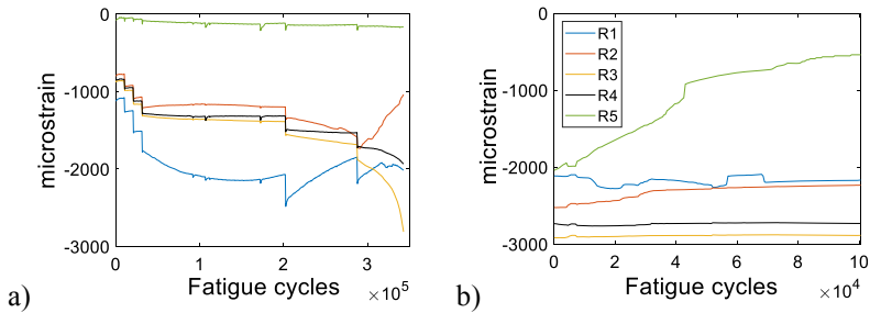
Fig. 2. Maximum FBG strains for a) L1_22 and b) L1_23 along the disbanded foot. (Similar legend for both figures)
