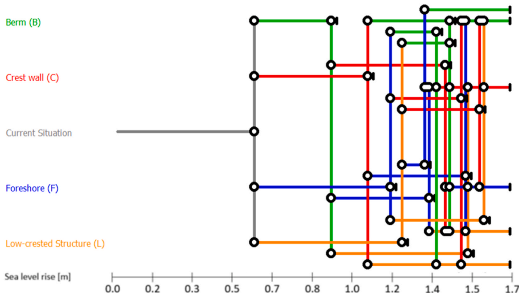
Fig. 2. Adaptation pathways for a rubble mound breakwater (from: Hogeveen, 2021).
