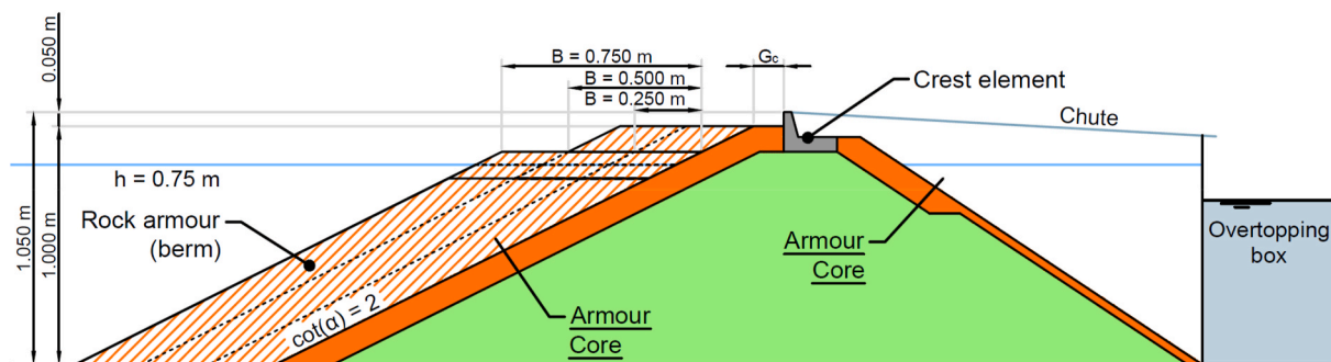
Fig. 4. Cross-sections of tested structures; Panel a: example of structure with filter layer (Configuration 2), Panel b: example of structure without a filter layer (Configuration 4).
