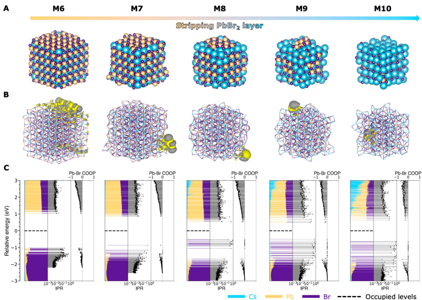
Figure 2. Formation of deep traps upon stripping of the PbBr 2 layer. (A) Structure, (B) isosurface plot of the HOMO, and (C) density of states (DOS), inverse participation ratio (IPR), and crystal orbital overlap population (COOP) of each model upon gradual stripping of the PbBr 2 layer. As shown in Figure S2 (models M1–M5), gradual stripping of the outer CsBr layer of our CsPbBr 3 model system does not create any trap states in the bandgap. However, upon removal of the underlying PbBr 2 layer (models M6–M10, shown here), deeper states start to appear. From model M8 onward, multiple deep traps, localized on surface Br − , are present.
