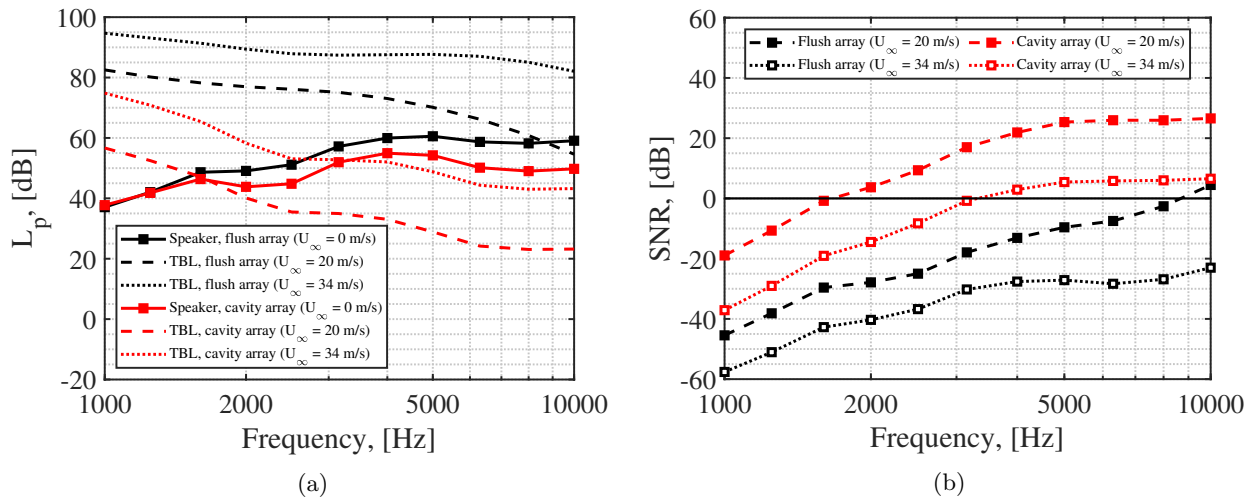
Figure 3: (a) Average one-third-octave band frequency spectra of the single speaker (without flow) as well as the TBL noise spectra (with speaker off) for the flow velocities of U_\infty = 20 m/s and 34 m/s for both array configurations. (b) Signal-to-noise ratio (SNR) of the speaker signal for both flow velocities and both array configurations.
