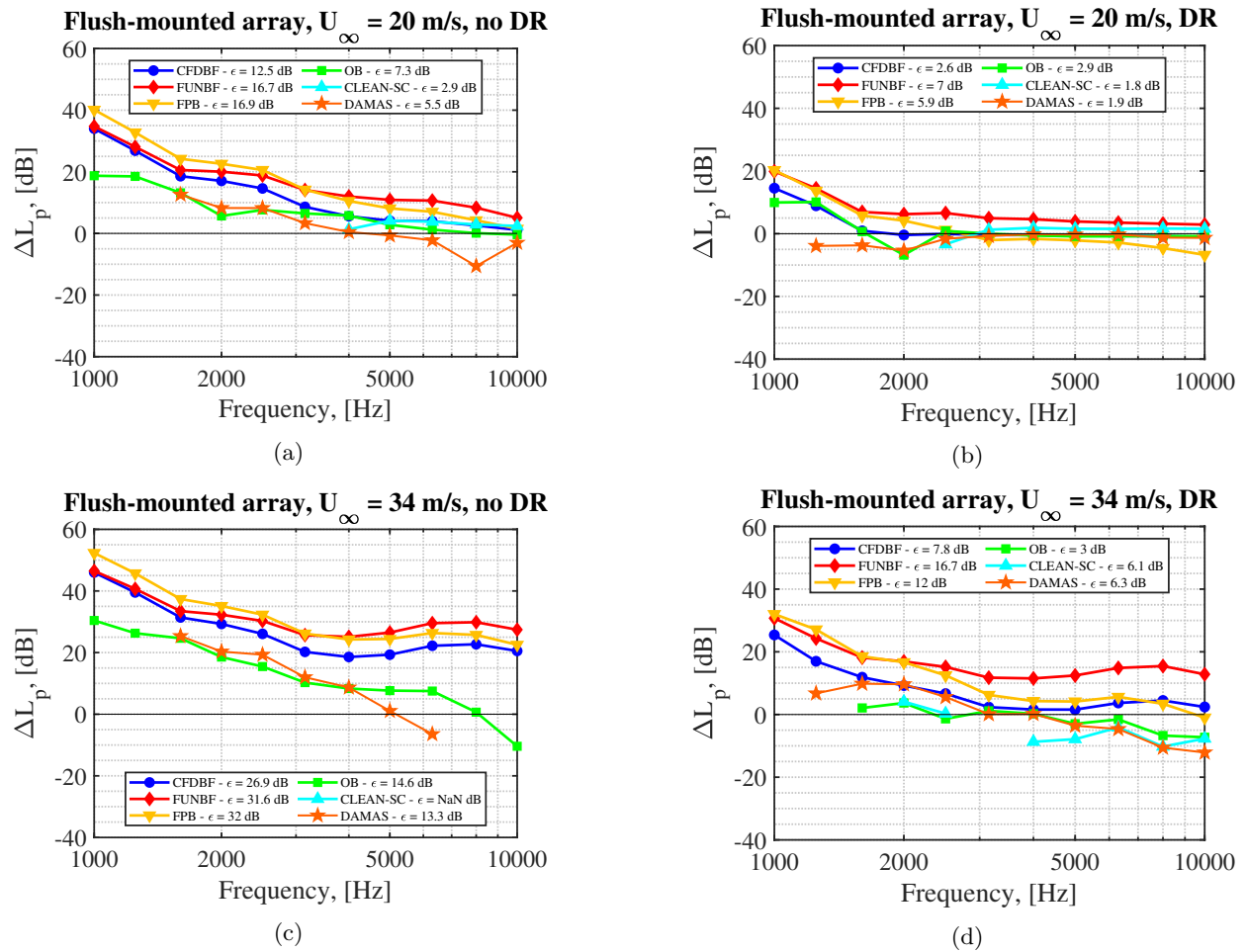
Figure 8: Relative errors made by each acoustic imaging method for the quantification of the sound emissions of the single speaker for the flush-mounted array for: (a) U_\infty = 20 m/s without DR, (b) U_\infty = 20 m/s with DR, (c) U_\infty = 34 m/s without DR, and (d) U_\infty = 34 m/s with DR.
