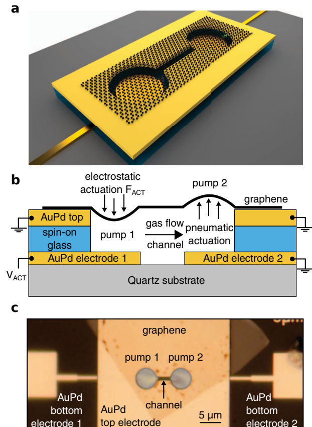
Figure 1: (a) A 3D schematic of the device: the graphene flake is covering two circular cavities that are connected through a narrow trench. (b) Schematic cross-section of the pumps and actuation mechanism for the case that pump 1 is actuated. (c) Optical micrograph of the device.
