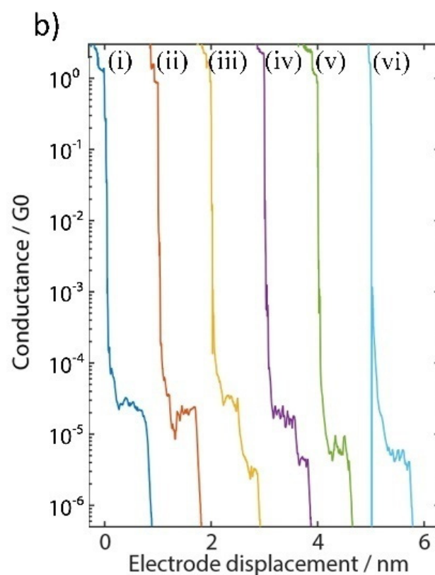
Figure 3. Individual breaking traces in presence of a molecule of: a) OxP 2: (i) empty junction, (ii) typical 'downhill' trace, (iii) single step plateau, (iv) double step plateau. b) (i-vi) Selected traces for reference compound 3. The traces are respectively offset along the x-axis by 1.2 and 1 nm for clarity.
