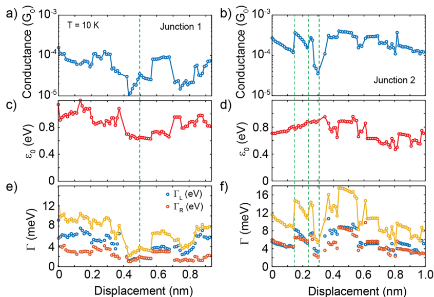
Figure 8. (a,b) Low-temperature conductance traces obtained from a low-bias fit of I – V s. (c,d) Corresponding level alignment and (e,f) electronic coupling during electrode separation as determined from fits to the Breit–Wigner model.
