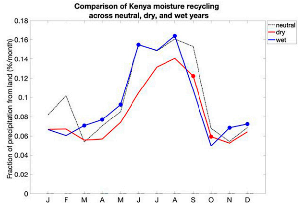
FIG. 4. Seasonal cycle of terrestrial moisture recycling in Kenya corresponding to wet, neutral, and dry conditions as defined by total annual precipitation (see section 2).
