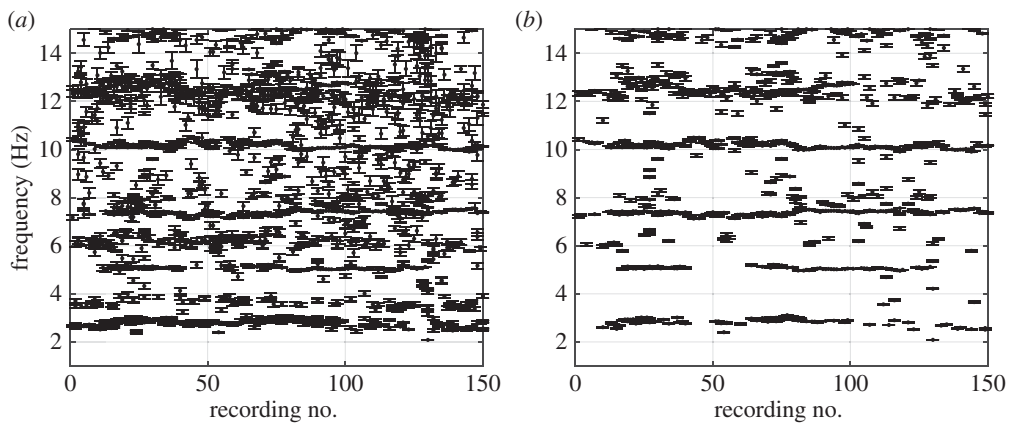
Figure 11. Identified frequencies and their uncertainties for each recording with two different tolerance values for the stabilization criterion: (a) tolerance criterion (\hat{\sigma}_{\omega_i} / \omega_i) < 0.03 and (b) tolerance criterion (\hat{\sigma}_{\omega_i} / \omega_i) < 0.01 .
