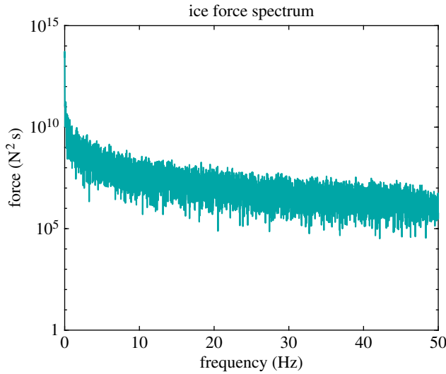
Figure 6. Ice force spectrum used for Monte Carlo simulations. (Online version in colour.)
