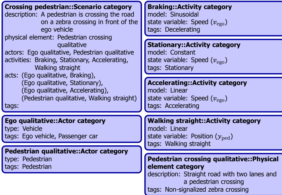
Figure 2.5: The objects that are used to qualitatively describe the scenario that is schematically shown in Figure 2.4. The first line of each block shows the name (before the double colon) and the class from which the object is instantiated. The following lines show the attributes of the object with the name and value of the attribute before and after the colon, respectively. For the sake of brevity, the unique ID of each object is omitted.
