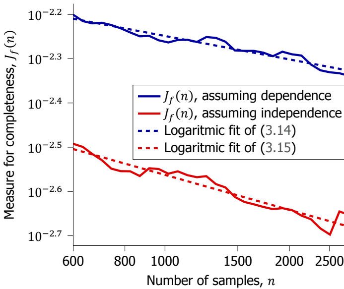
Figure 3.6: The measures of completeness for the example of Section 3.4.2 with the assumption that all three parameters depend on each other (blue solid line) and with the assumption that the first parameter, i.e., the average deceleration, does not depend on the other two parameters (red solid line). The corresponding dashed lines represent the least squares logarithmic fits given by (3.14) and (3.15).
