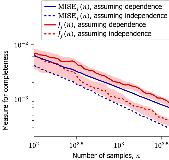
Figure 3.3: The real MISEs (blue lines) of the example of Section 3.4.1, approximated using (3.13), and the measures that are used to quantify the completeness (red lines). The solid lines show the result of estimating a bivariate pdf, so here (3.8) is used to quantify the completeness. The dashed lines show the result of estimating two univariate pdfs and combining them according to (3.10) to create a bivariate pdf, so (3.12) is used to quantify the completeness. The red areas show the interval [\mu - 3\sigma, \mu + 3\sigma] , where \mu and \sigma denote the mean and standard deviation, respectively, of the measures of (3.8) and (3.12) when repeating the experiment 200 times.
