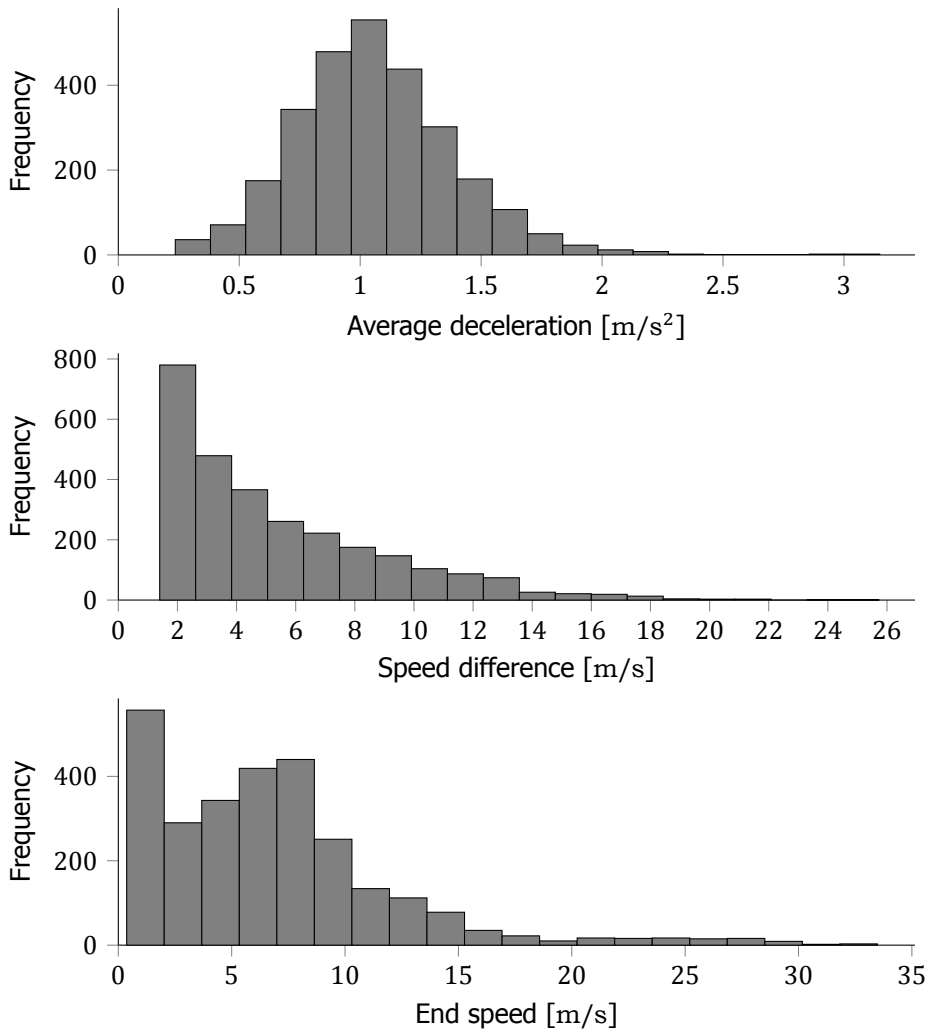
Figure 3.4: Histograms of the data that are used for the example of Section 3.4.2.
