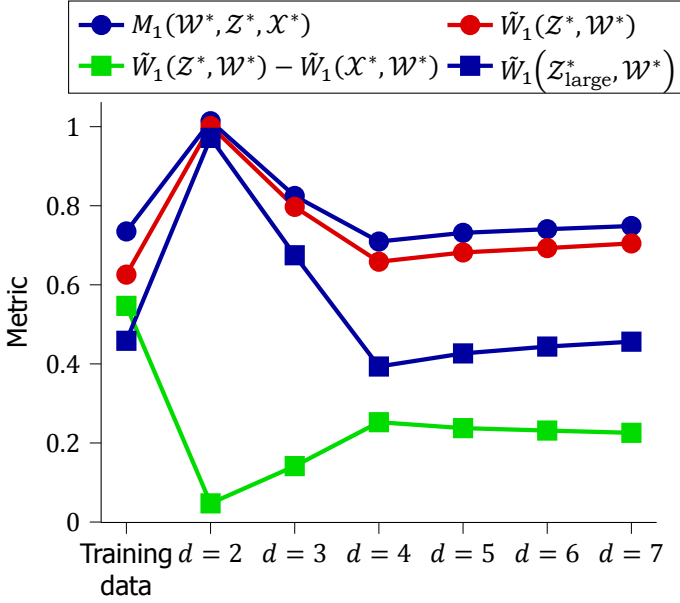
Figure 5.9: Medians of the metrics for the set of N_w = 10000 generated LVD scenario parameter vectors. In this case, the N_x = 920 scenarios of \mathcal{X}^* are sampled from \hat{f}_H(\cdot) of (5.11), where \hat{f}_H(\cdot) is based on the original data set \mathcal{X} .
