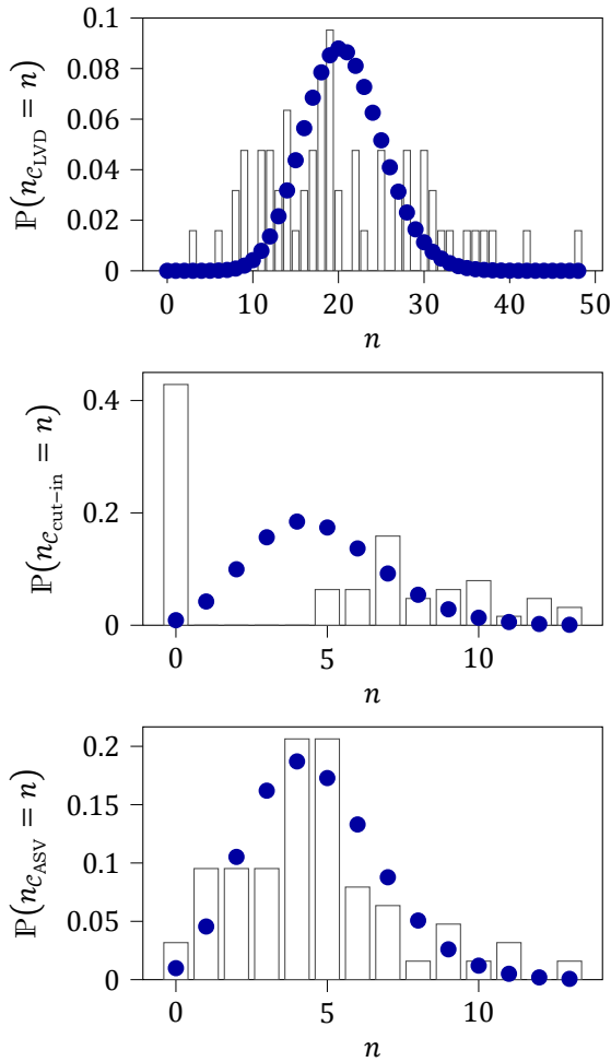
Figure 7.5: The bar graph shows how often a scenario of scenario category C_{LVD} , C_{cut-in} , or C_{ASV} is encountered n times per hour of driving divided over the total number of hours, 63. For comparison, the dots denote the Poisson distribution of (7.2) with the maximum likelihood estimate of \lambda .
