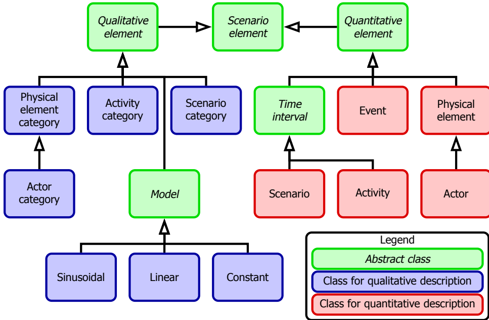
Figure 2.2: Class-level relationships of most classes of our Object-Oriented Framework (OOF).
