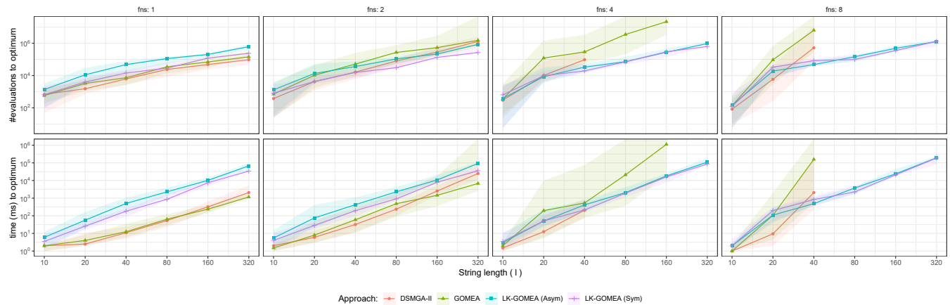
Figure 3: Scalability in number of evaluations (top) and time in ms (bottom) on BoT for various problem sizes (i.e. string lengths l ) and number of subfunctions fns . The line represents the median, whereas the shaded area ranges from the 95th percentile to the 5th percentile. If the median run was unable to find the optimum within the allotted budget, the point is left out.
