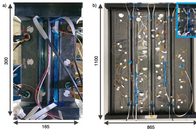
Figure 1. Two stiffened sensorized panels used in the upscaling study: a) single-stiffener panel and b) multi-stiffener panel, including their dimensions in mm. Note that the main images of a) and b) are not to scale. Therefore, to indicate the dimensionality change between the two panels, b) includes a to-scale image of the single-stiffener coupon.
