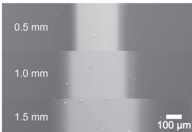
Figure 6. Compound SEM image (taken at 5 kV) of three lines printed after each other with nozzle distances of 0.5 mm, 1.0 mm, and 1.5 mm. The deposition rate of the nozzle is assumed constant as these lines are printed immediately after each other with identical settings. Provided the impaction efficiency remains the same for all distances, the mass of each line should be equal.
