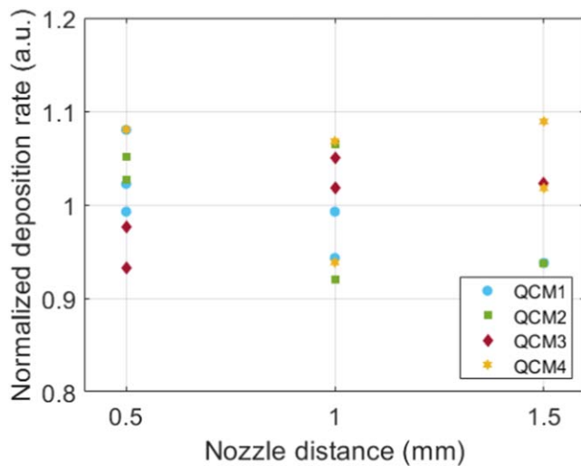
Figure 5. Deposition rate as a function of nozzle distance. Per QCM, all data was collected in the same synthesis session to minimize fluctuations between depositions. The data points are normalized to the mean per QCM for better comparison.
