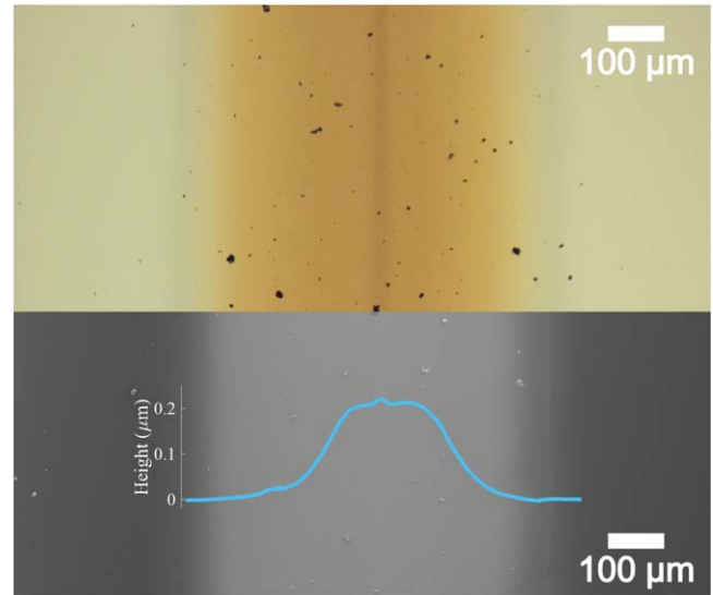
Figure 7. Compound image of an optical and scanning electron microscope image (taken at 5 kV) of a printed line on an Al surface. The profile in blue is an average of two Dektak profile measurements on two separate places with the peak at its approximate location overlaid on the image and with the same scale as the SEM image on its horizontal axis. Nozzle distance of 1 mm, 0.5 mm min -1 , writing speed, 5 mA generator current.
