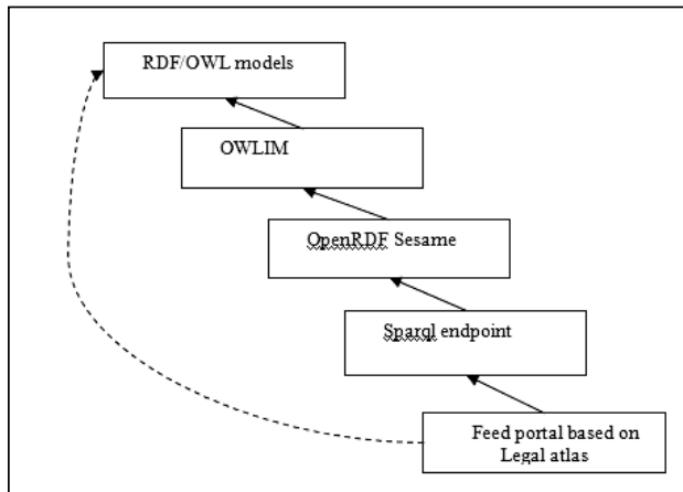
Figure 4: Architecture of the annotation engine of a map based conflict resolution portal.
