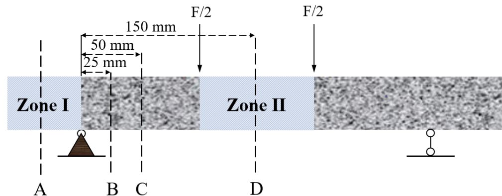
Figure 2. Schematic view of the carbonation depth measurement.
