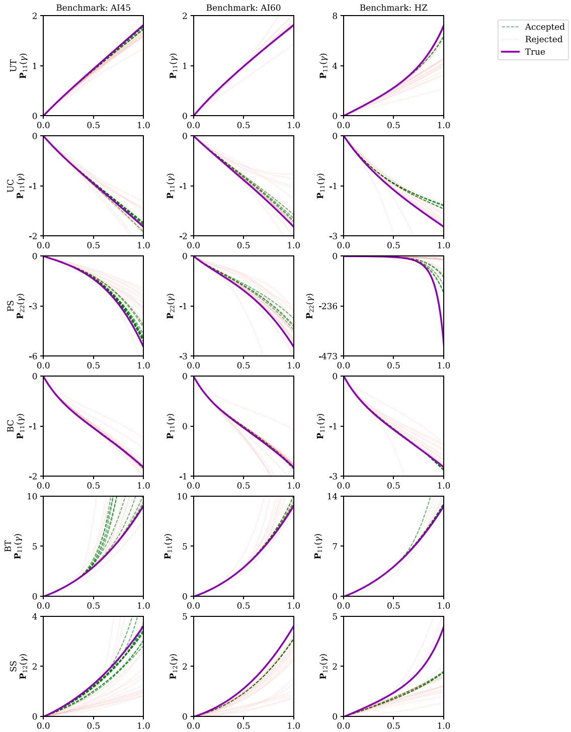
Fig. C.14. First Piola-Kirchhoff stress P(F(\gamma)) component prediction along the different deformation paths in (33) using the ICNN-based constitutive models (both accepted and rejected ones) for the case with low noise ( \sigma_u = 10^{-4} ) and benchmarks AI45 (29), AI60 (30), and HZ (31). The constitutive response of the (hidden) true model is also shown for reference.
