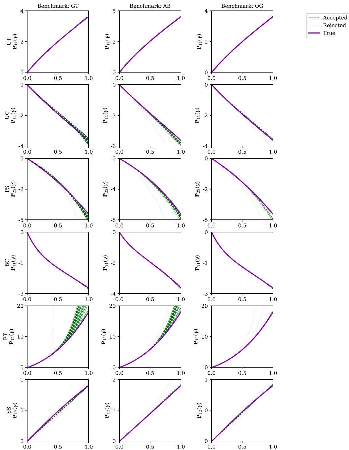
Fig. C.13. First Piola-Kirchhoff stress P(F(\gamma)) component prediction along the different deformation paths in (33) using the ICNN-based constitutive models (both accepted and rejected ones) for the case with low noise ( \sigma_u = 10^{-4} ) and benchmarks GT (26), AB (27), and OG (28). The constitutive response of the (hidden) true model is also shown for reference.
