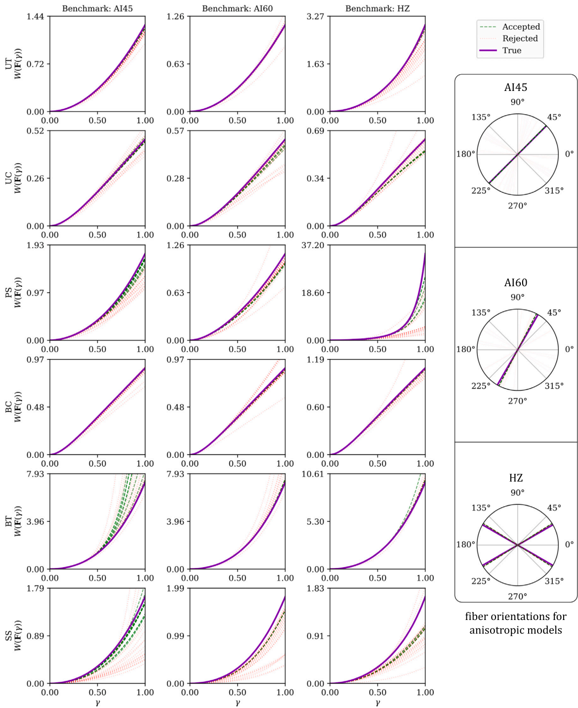
Fig. 6. Strain energy density W(\mathbf{F}(\gamma)) prediction along the different deformation paths in (33) using the ICNN-based constitutive models (both accepted and rejected ones) for the case with low noise ( \sigma_u = 10^{-4} ) and benchmarks AI45 (29), AI60 (30), and HZ (31). The constitutive response of the (hidden) true model is also shown for reference. The insets show the fiber orientations discovered by the ICNN-based models and the fiber orientations in the (hidden) true model.
