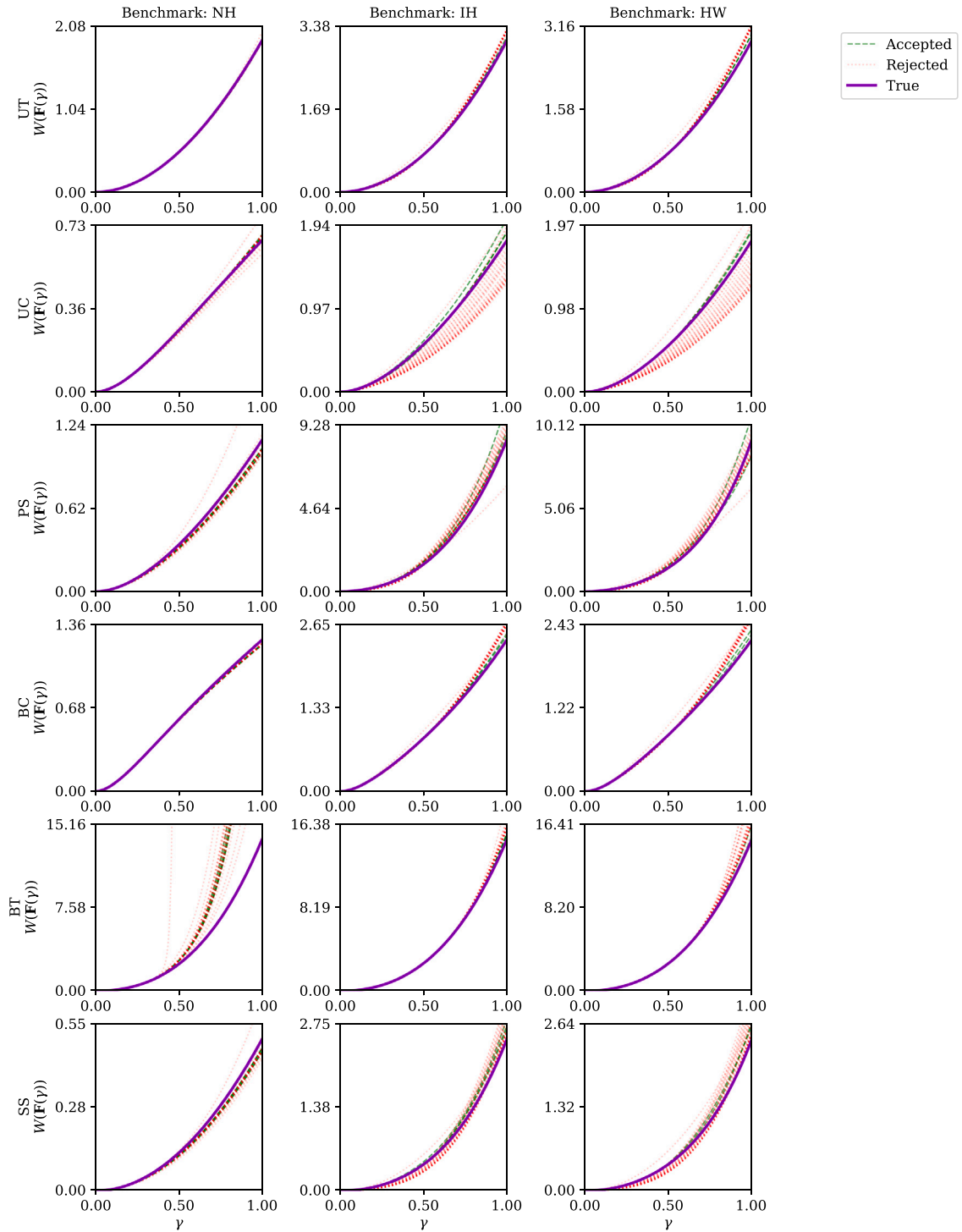
Fig. 4. Strain energy density W(\mathbf{F}(\gamma)) prediction along the different deformation paths in (33) using the ICNN-based constitutive models (both accepted and rejected ones) for the case with low noise ( \sigma_u = 10^{-4} ) and benchmarks NH (23), IH (24), and HW (25). The constitutive response of the (hidden) true model is also shown for reference.
