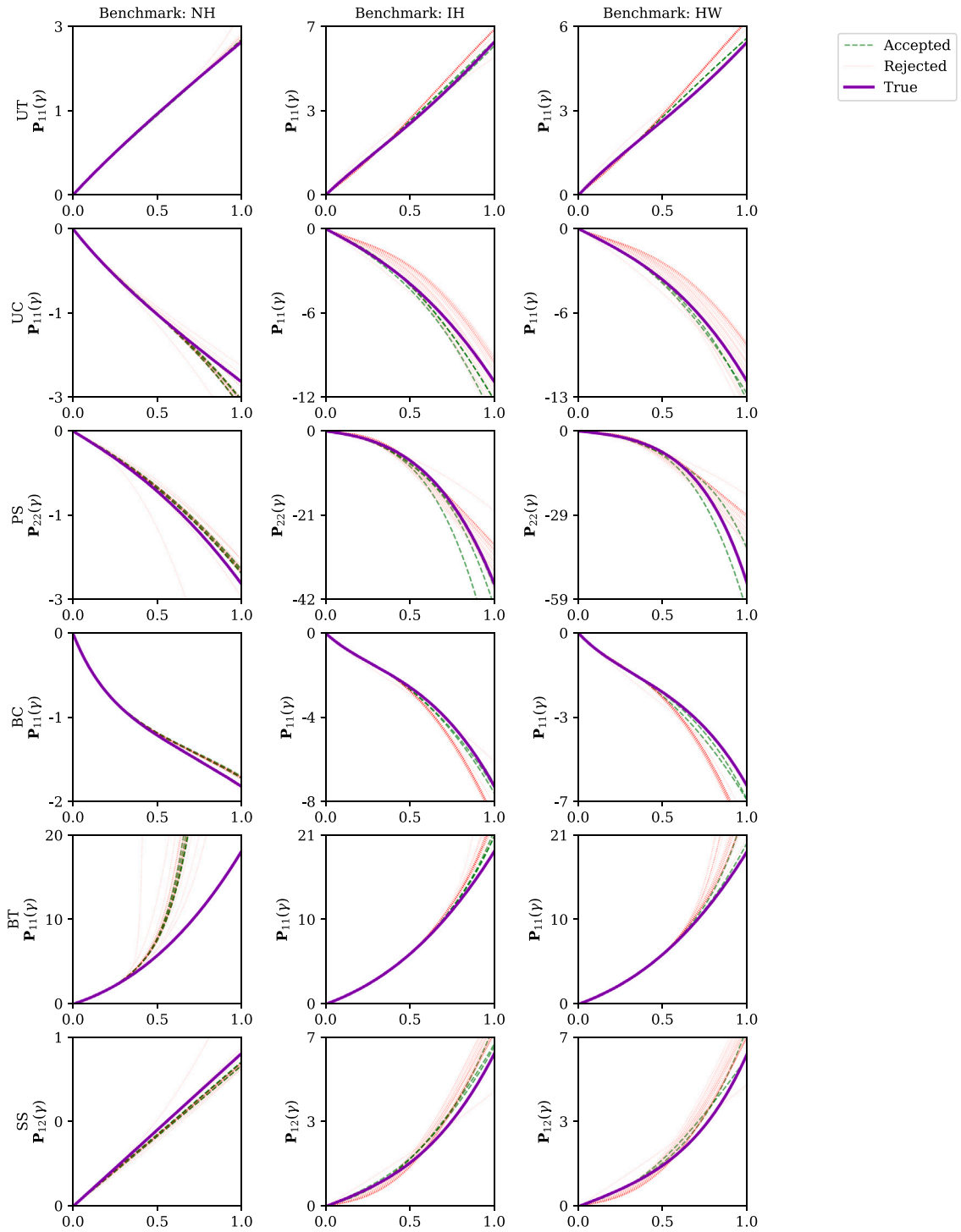
Fig. C.12. First Piola-Kirchhoff stress P(F(\gamma)) component prediction along the different deformation paths in (33) using the ICNN-based constitutive models (both accepted and rejected ones) for the case with low noise ( \sigma_u = 10^{-4} ) and benchmarks NH (23), IH (24), and HW (25). The constitutive response of the (hidden) true model is also shown for reference.
