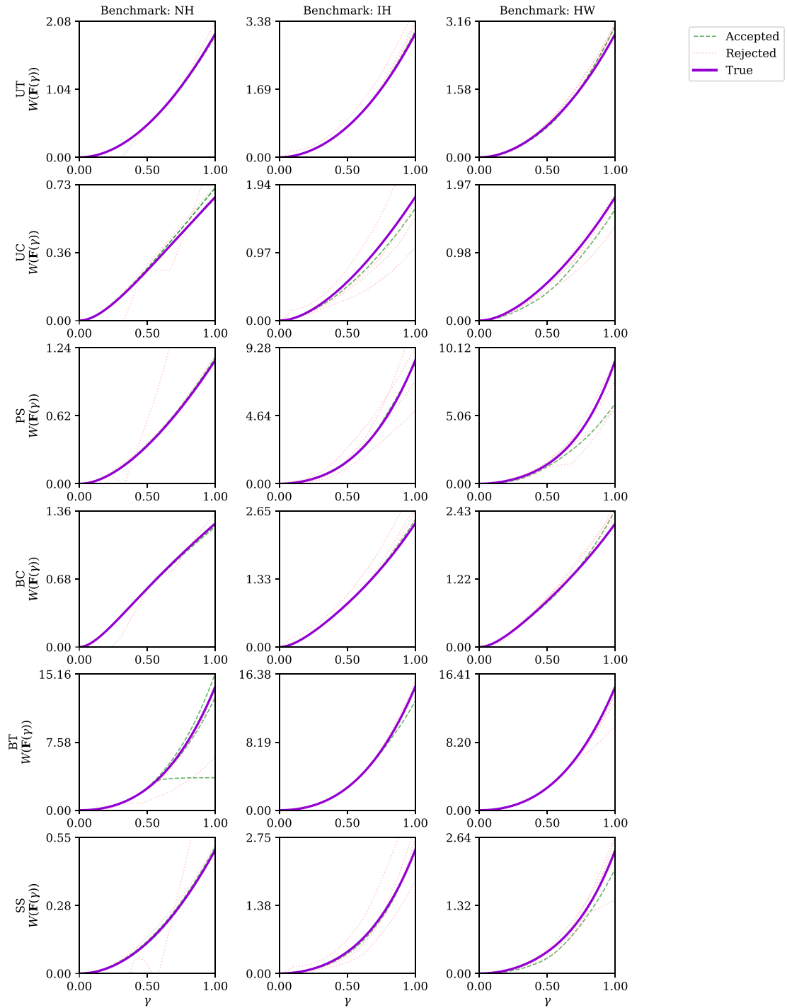
Fig. D.18. Strain energy density W(\mathbf{F}(\gamma)) prediction along the different deformation paths in (33) using the NN-based (non-convex and non-smooth) constitutive models (both accepted and rejected ones) for the case with high noise ( \sigma_u = 10^{-3} ) and benchmarks NH (23), IH (24), and HW (25). The constitutive response of the (hidden) true model is also shown for reference.
