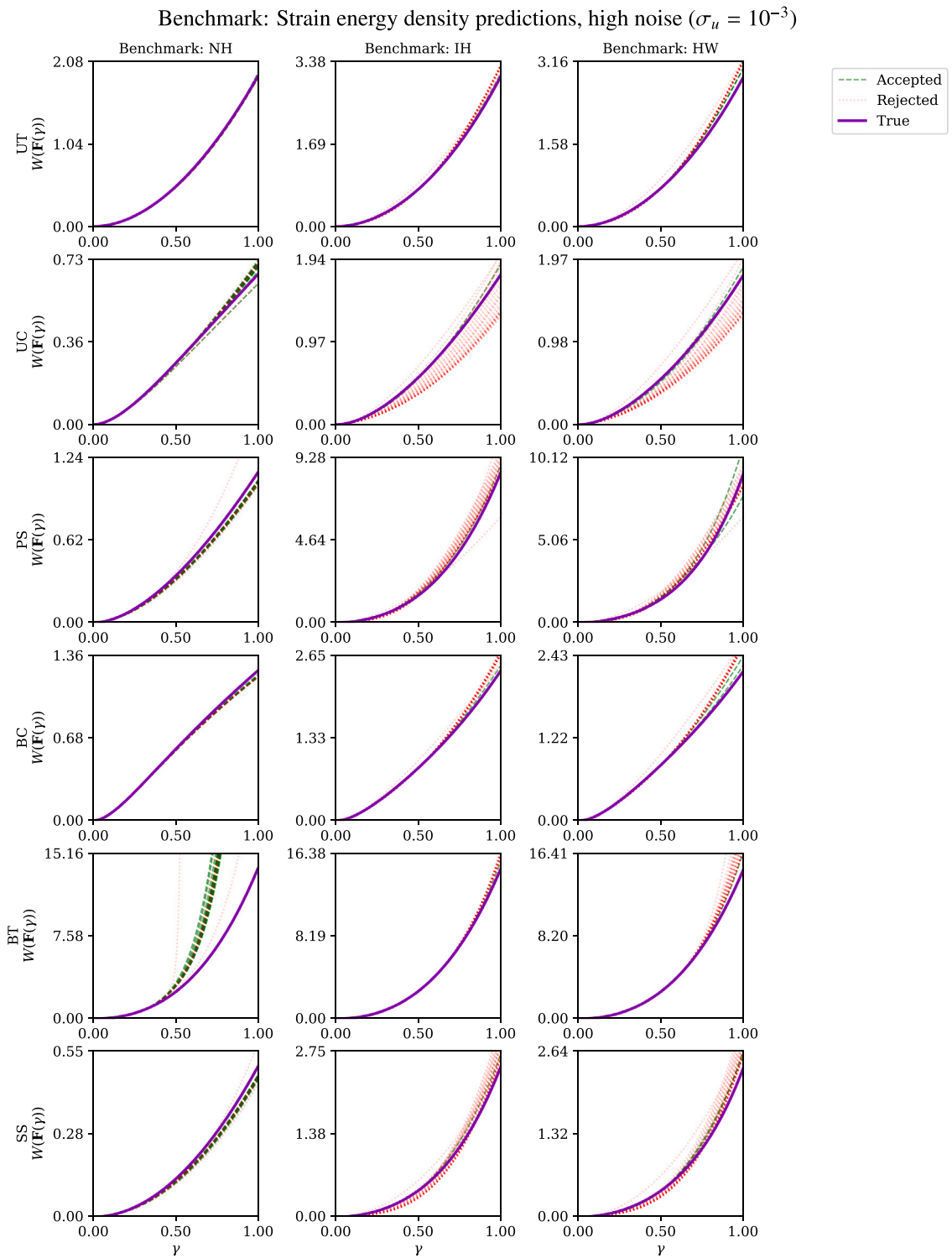
Fig. 7. Strain energy density W(F(\gamma)) prediction along the different deformation paths in (33) using the ICNN-based constitutive models (both accepted and rejected ones) for the case with high noise ( \sigma_u = 10^{-3} ) and benchmarks NH (23), IH (24), and HW (25). The constitutive response of the (hidden) true model is also shown for reference.
