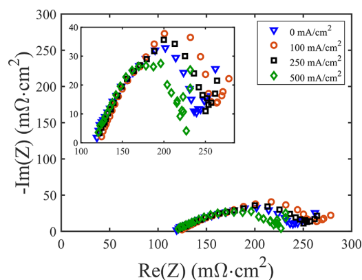
Figure 6. Measured impedance of our membraneless \text{H}_2\text{-Br}_2 battery, in the form of a Nyquist plot. Impedance is shown for various DC current values including 0 (blue triangles), 100 (red circles), 250 (black squares) and 500 \text{ mA/cm}^2 (green diamonds). Inset shows a zoom-in view of the measured impedance.
