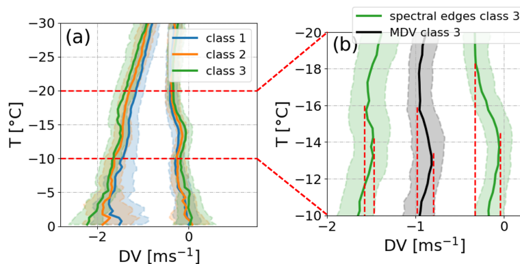
Figure 5. (a) Derived Doppler velocities of the spectral edges classified into \text{DWR}_{\text{KaW}} classes (see also Table 2). Solid lines indicate the median and the shading denotes the quantiles of the distribution. The dashed red lines indicate the location of the DGL. (b) Zoomed view into the DGL region but only including the spectral edge velocities (green) and MDV (black) of class 3. The vertical dashed red lines in (b) visualise the points in the spectral edges and MDV which have been used to estimate the maximum velocity reduction (see details in the text).
