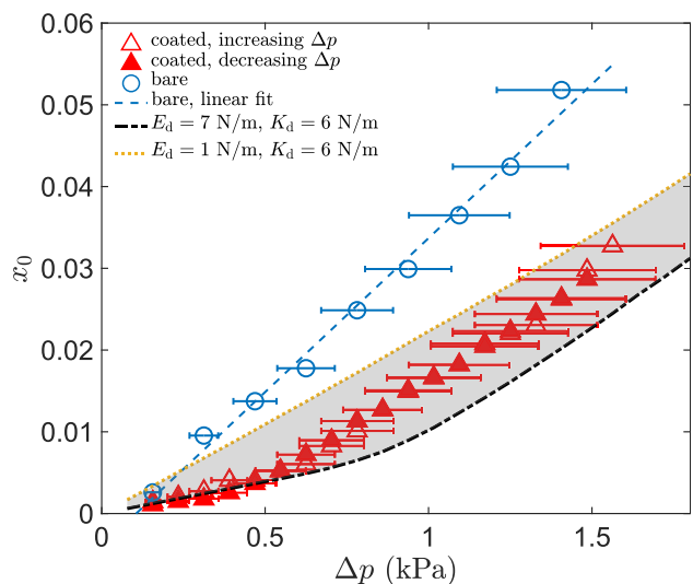
Fig. 5. Pressure sweep on colloid-coated bubbles. A coated bubble, with R_0 = 134.7\mu\text{m} and coated by 2a = 5\mu\text{m} colloids, is subjected to increasing acoustic pressures (open red triangles) and then to decreasing pressures (filled red triangles). For comparison, experimental results for a bare bubble of the same radius (open blue circles) is shown for each case, with the linear fit to the data (blue dashed line). The error bars on x_0 are smaller than the symbols. Model predictions are shown for high estimate of E_d = 7\text{N/m} (black dotted-dashed line) and lower estimate of E_d = 1\text{N/m} (orange dotted line). In both cases K_d = 6\text{N/m} . The coated bubble data lie between these two theoretical bounds, as shown by the shaded region.
