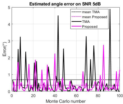
Fig. 5. The Monte Carlo test results with low SNR (5dB)
