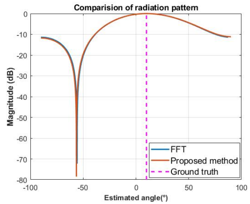
Fig. 3. The comparison of radiation patter between FFT and proposed method.
