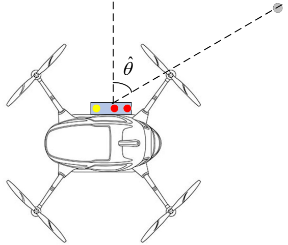
Fig. 1. The assumed scenario for side-mounted UAV radar; the transmitter is marked in yellow, while the receivers are marked in red.
