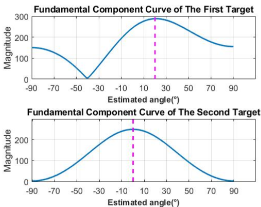
Fig. 6. The fundamental component curves of 2 different targets
