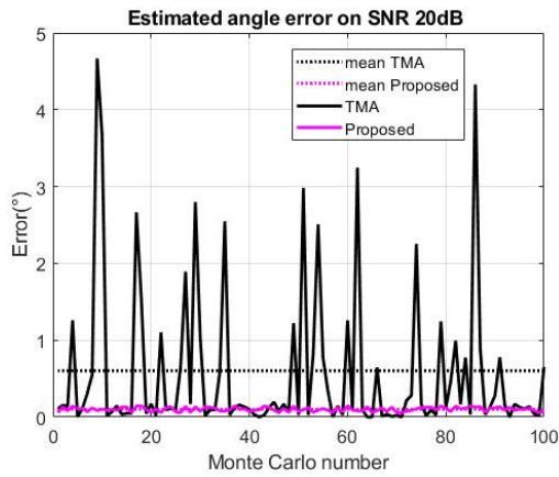
Fig. 4. The Monte Carlo test results with high SNR (20dB)
