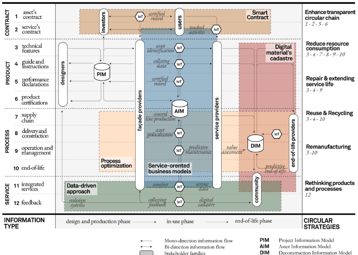
Fig. 3. IoT-enabled framework for circular façade information flows.
