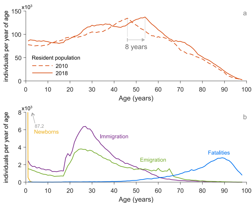
Figure 3. Age distribution of the Swiss resident population in 2010 and 2018 (a) and of the Swiss input/output population fluxes in 2018 (b). All these age distributions are different and change over time because they reflect different physical and social processes. Data from the Swiss Federal Statistical Office. Age distributions have a resolution of 1 yr.
