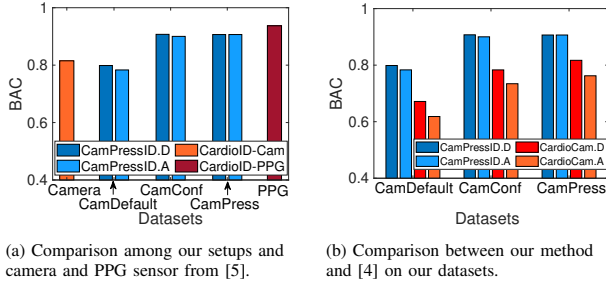
Figure 10: Comparison among our method, [5] and [4]. CamPressID.D/A stand for results with detectable/all subjects in CamPressID. CardioCam.D/A stand for results with with detectable/all subjects in [4].
