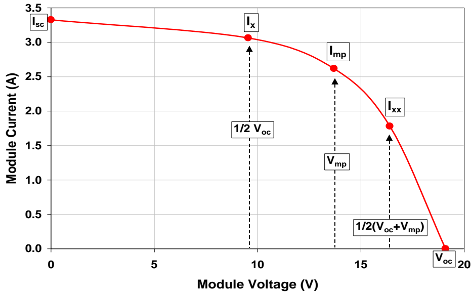
Figure 55: Model points on the IV curve described by the Sandia Array Performance Model (reproduced from [45]).
