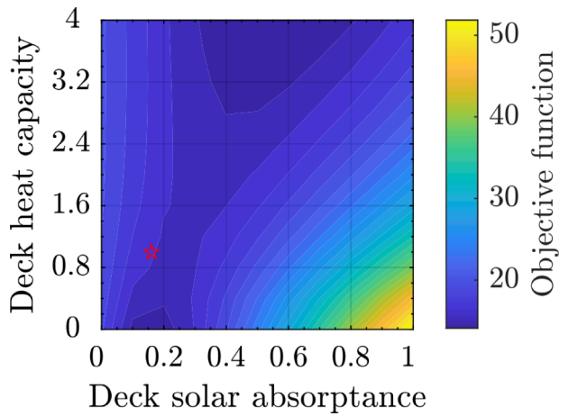
(a) Deck heat capacity vs. Deck solar absorptance
