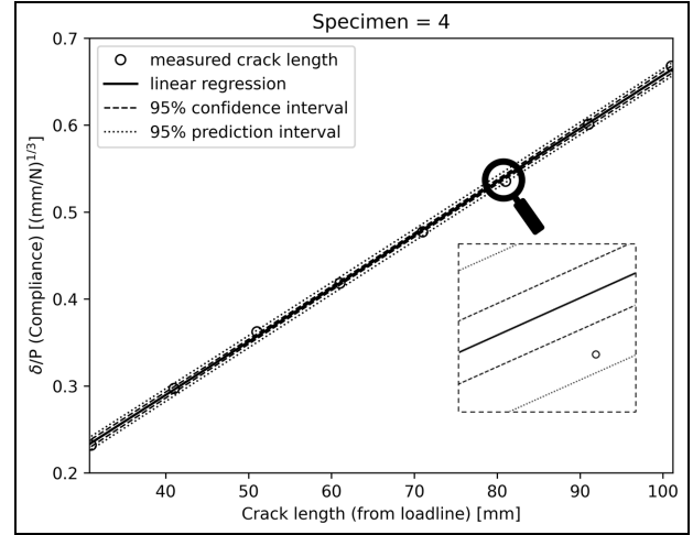
Figure 5. Compliance calibration.
