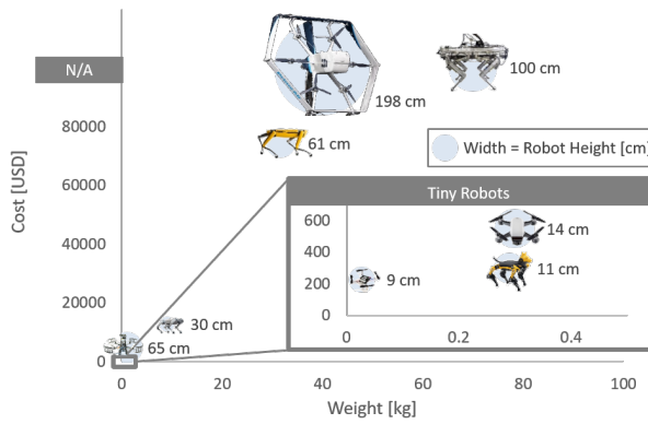
Fig. 2. Tiny robots are resource-constrained low-cost autonomous robots. Pictured are full-size [3], [7], [18], [23], [46] and tiny [6], [13], [40] robots.
