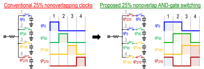
Fig. 2. The AND-gate switching N-path filter’s principles.
