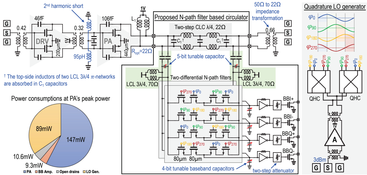
Fig. 3. The top-level view of the mm-wave FD/FDD TRX front-end and its power consumption at PA's peak power.
