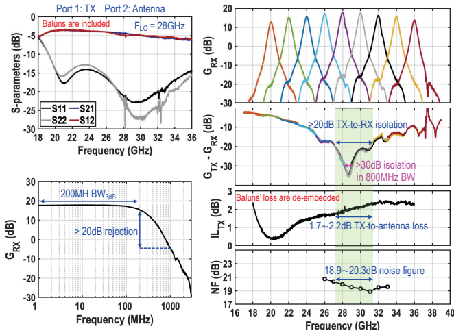
Fig. 5. Small-signal s-parameter, RX gain, TX-to-RX isolation, noise figure, and TX-to-antenna insertion loss over the 20-to-36GHz band.
