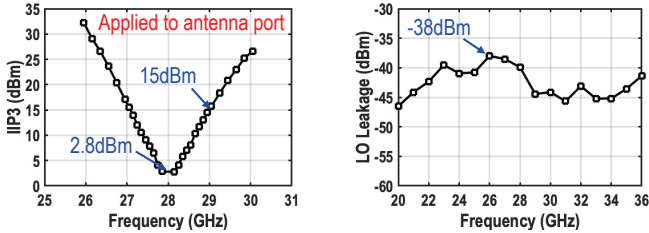
Fig. 10. The measured IIP 3 and LO leakage.
