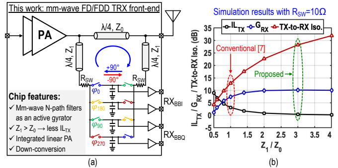
Fig. 1. (a) The proposed mm-wave FD/FDD TRX front-end architecture and (b) simulation results of TX insertion loss, RX gain, and TX-to-RX isolation versus characteristic impedance of gyrator’s QTLs.
