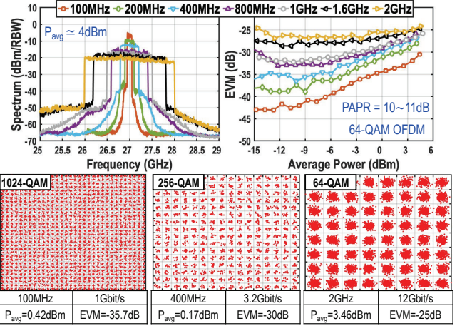
Fig. 7. The OFDM signal measurement results of the TX path.
