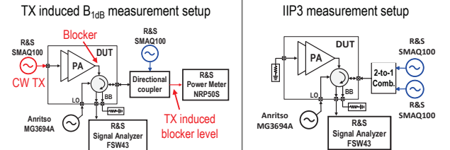
Fig. 8. The measurement setups of the TX induced B_{1dB} and IIP 3 .
