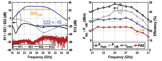
Fig. 6. Small-signal s-parameter and large-signal CW measurement results of the TX path.
