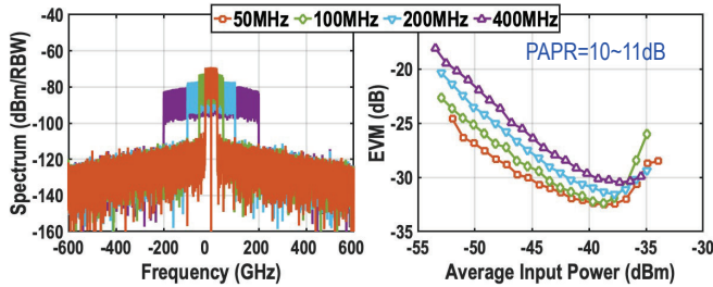
Fig. 11. The OFDM signal measurement results of the RX path.
