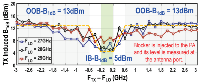
Fig. 9. The measured TX induced B_{1dB} at various carrier frequencies.
