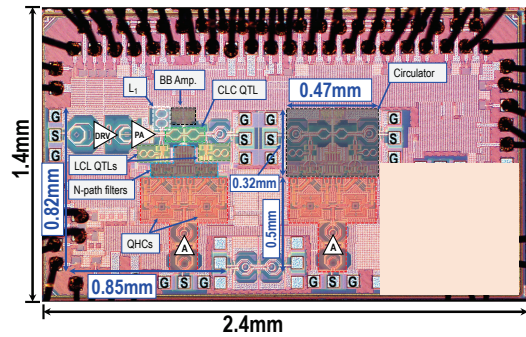
Fig. 4. Die micrograph of the proposed FD/FDD TRX front-end.
