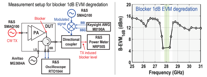
Fig. 12. The RX EVM degradation under the OOB CW TX blocker measurement setup and results.
