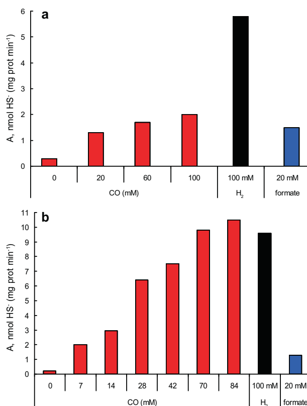
Fig. 3 Sulfidogenic activity of resting cells of carboxydutrophic haloarchaea grown anaerobically with CO and sulfur. (a) HSR-CO; (b) AArc-CO. Cells of HSR-CO were incubated in 4 M NaCl containing 50 mM K-P buffer at pH 7. Cells of AArc-CO were incubated in an alkaline buffer containing 3.5 M NaCl and 0.5 M Na^+ as sodium carbonates, pH 9.5. The incubation temperature was 30 °C. The anoxic cell suspensions were reduced by 0.2 mM sulfide and 10 \mu l of 10% dithionite in 1 M NaHCO_3 /2 ml. The chemical controls were buffers without cells and were negative during the whole incubation period (up to 7 days). The data are mean values from duplicate experiments.
