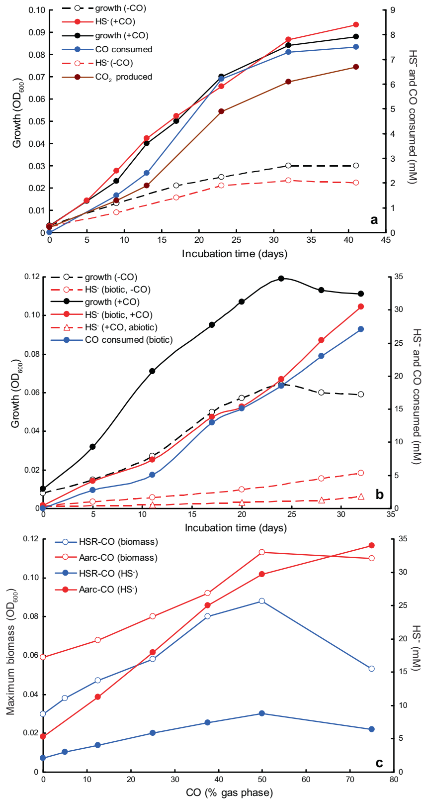
Fig. 2 Anaerobic growth kinetics of carboxydotrophic sulfur-reducing haloarchaea grown at 4.0 M total Na + /pH 7/37 °C (HSR-CO) or pH 9.5/30 °C (Aarc-CO) with 0.5 g l -1 yeast extract as the carbon source, CO as the electron donor and elemental sulfur as the electron acceptor. a , b , growth dynamics at 55 mM CO; ( c ), influence of CO concentration on growth and sulfur-reducing activity. The data are mean values from three parallel incubations.
