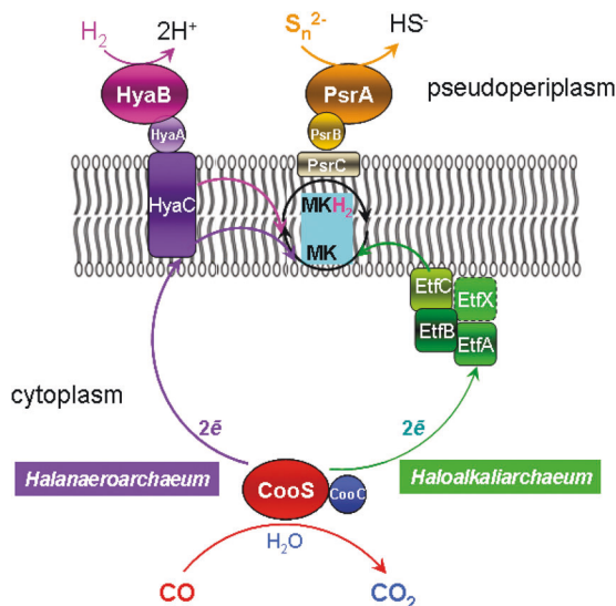
Fig. 5 Hypothetical scheme of electron transport from CooS to PsrABC in two anaerobic carboxydutrophic haloarchaea (based on genomic content). HyaABC membrane-bound Ni, Fe uptake hydrogenase, PsrABC membrane-bound polysulfide reductase, EtfABCX cytoplasmic electron transfer flavoprotein complex, MK/MKH2 menaquinone-menaquinol, S polysulfide.
