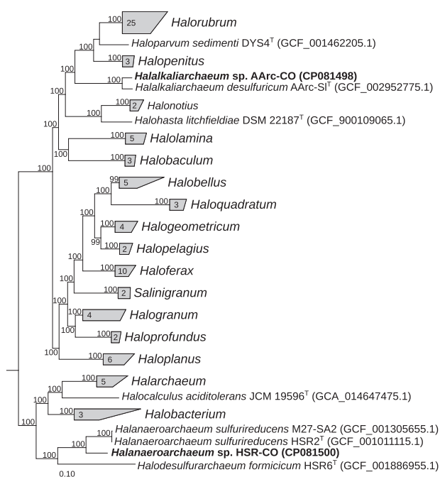
Fig. 1 Phylogenomic placement of carboxydophilic sulfur-reducing isolates AArc-CO and HSR-CO among their nearest relatives based on maximum likelihood inference and concatenated partial amino acid sequences of 122 archaeal single copy conserved marker proteins. Bootstrap consensus tree is shown with values above 90% placed at the nodes. Bar, 0.1 changes per position.
